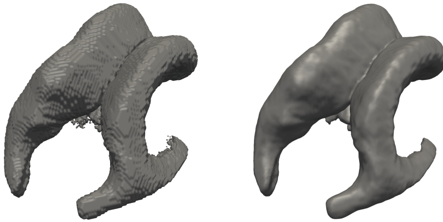
Fig. 2. Lateral ventricles of a human brain, segmented from an MR volume image using 20 single-voxel seed-points. A polygonal surface was extracted from the segmented volume using the Marching Cubes algorithm [13], which takes sub-pixel information into account (Left) Segmentation obtained by the IFT. (Right) Segmentation obtained by the sub-pixel IFT proposed in [8].
